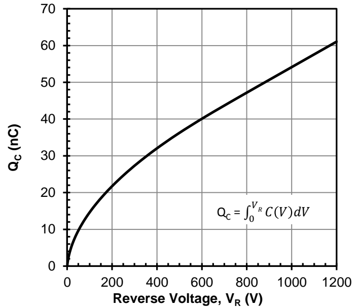
Figure 4 Typical capacitive charge vs. reverse voltage
