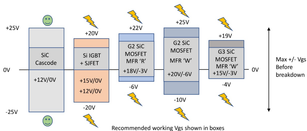
Figure 6. SiC cascodes encompass other allowable gate-drive voltage ranges
