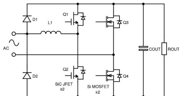
Figure 10. SiC devices in a bridgeless totem-pole PFC stage
