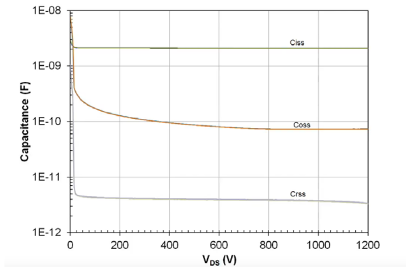
Figure 3. Typical SiC cascode device capacitances
